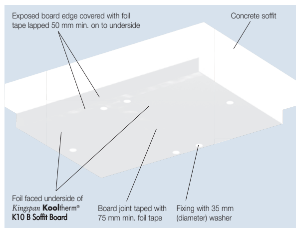
Figure 2 – Protection of Exposed Insulation Edges of Kingspan Kooltherm® K10 B Soffit Board .
